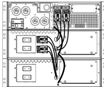
Battery Connections
