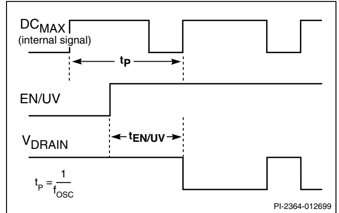
Figure 18. Output Enable Timing.
